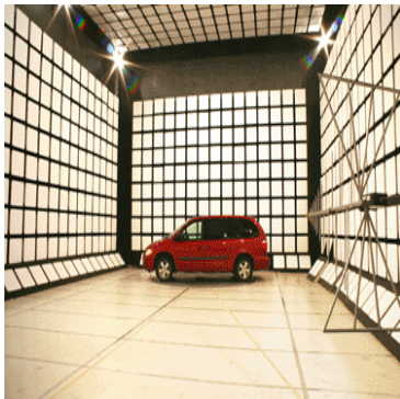
10 meter TDK chamber
